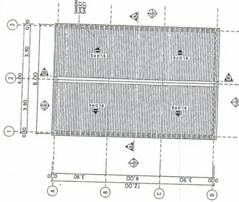
2 ROOF PLAN SCALE 1:100 DATE 11/08/2018
